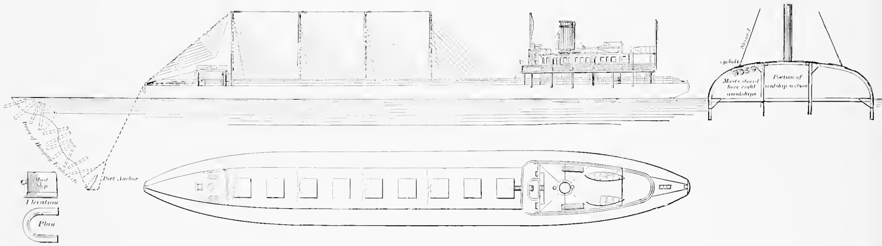
WHALEBACK STEAMER CHAS. W. WETMORE, SHOWING JURY MASTS STEPPED.
